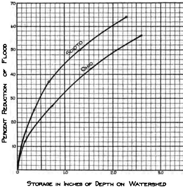
FIG. 40.—Diagram showing relation between amount of storage and flood reduction on Ohio River at Cincinnati (75,800 sq. mi.), and Scioto River at Columbus storage dam (1,053 sq. mi.).
